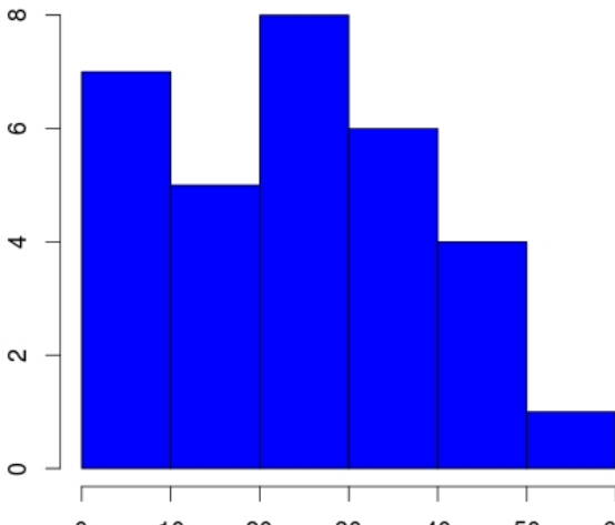
Histogram of sample
